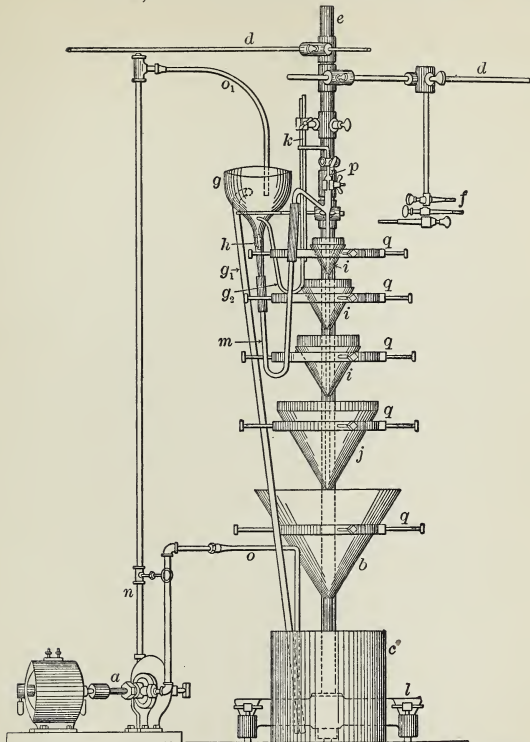
FIG. 41.—Thompson's Classifier, for Pigments and Fine Particles in General.
